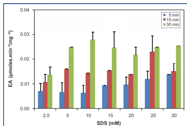
Figure 2. Effect of SDS concentration on PO activity in P. pythagoricus . The dependence of activation on different concentrations of SDS (2.5–30 mM; final concentrations) was assayed in 100 mM sodium phosphate buffer (pH 7.5) at 25°C. The Hc concentration was 0.3 mg/mL and 1 mM dopamine was used as substrate. First, Hc was preincubated with SDS for 5, 15, and 30 min; then the reaction was started by the addition of substrate. The reaction was followed by measuring the absorption at 475 nm.
