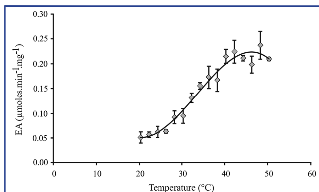
Figure 4. Effect of temperature on PO activity in P. pythagoricus . Values represent the mean \pm one SD, n = 3 .
