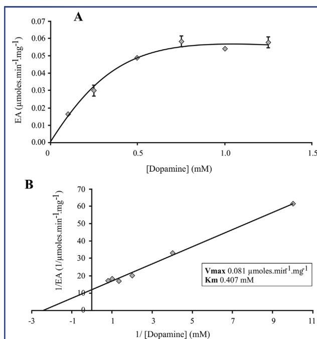
Figure 3. Kinetic analysis of PO activity in P. pythagoricus . A: The enzymatic activity of P. pythagoricus Hc (0.3 mg/mL) was assayed at an SDS concentration of 10 mM in 100 mM sodium phosphate buffer, pH 7.5 at 25°C. P. pythagoricus Hc was incubated with SDS for 30 min before addition of the dopamine substrate. B: Representation of Lineweaver–Burk of the effect of dopamine concentration on PO activity in P. pythagoricus . V_0 : initial velocity. K_m : 0.407 mM, V_{max} : 0.081 \mu\text{mol} \cdot \text{min}^{-1} \cdot \text{mg protein}^{-1} . Hill Coefficient \sim 1 . Results are means \pm SEM of three independent determinations.
