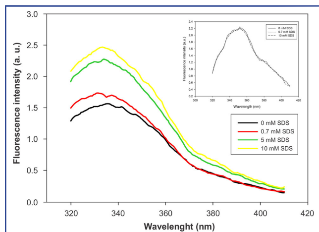
Figure 6. Fluorescence emission spectra of 0.1 mg/mL P. pythagoricus Hc in 100 mM sodium phosphate buffer, pH 7.5, excited at 290 nm, after 30 min incubation in SDS across the range 0, 0.7 and 5 and 10 mM. Inset: Fluorescence emission spectra of 2 \mu M N-acetyl tryptophan in 100 mM sodium phosphate buffer pH 7.5, excited at 290 nm, in the absence of SDS and following 30-min incubation in 0.7 mM and 10 mM SDS.
