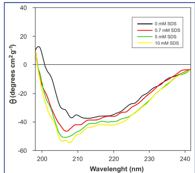
Figure 5. Far UV CD spectra of 8 mg/mL P. pythagoricus Hc in 100 mM sodium phosphate buffer, pH 7.5, after 30-min incubations with SDS across the range 0, 0.7 and 5 and 10 mM.
