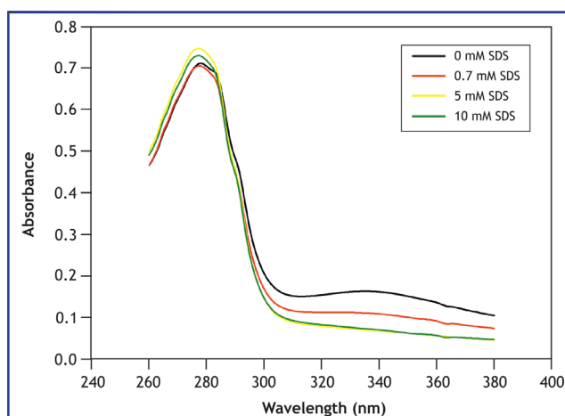
Figure 7. Absorption spectra of 0.3 mg/mL P. pythagoricus Hc in 100 mM sodium phosphate buffer, pH 7.5, after 30-min incubation at different concentrations of SDS (0, 0.7, 5 and 10 mM).
