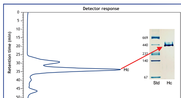
Figure 1. Chromatographic profile from FPLC obtained during purification of Hc from the P. pythagoricus hemolymph isolated by ultracentrifugation, on a Superdex-200 column equilibrated and eluted with 100 mM Tris-HCl, containing 10 mM \text{CaCl}_2 , 50 mM \text{MgCl}_2 , pH 8, at a 0.4 mL/min flow rate. The highest peak is hexamer of Hc. Inset: Native-PAGE profile of the highest peak isolated from FPLC.
