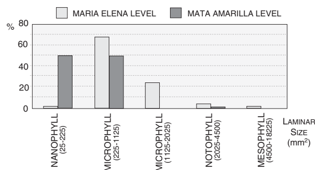
TEXT-FIG. 13. Comparative laminar size in the plant-bearing levels based on 164 measurements. Microphyll leaf size was divided into two size categories in order to delimit the two data populations more clearly: one between 225 and 1125 mm 2 and the other between 1125 and 2025 mm 2 .
