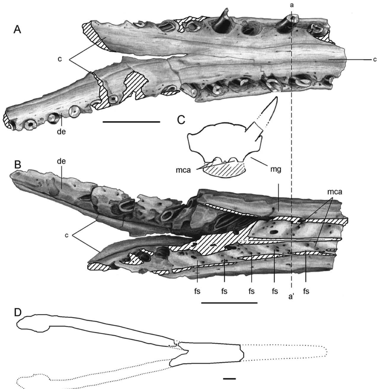
Fig. 7. Sulcusuchus erraini (MPEF 650). Interpretative drawings. Mandibular symphysis in A , dorsal and B , ventral views; C , reconstructed cross-section aa'; D , schematic reconstruction of mandible showing the position of the preserved left mandibular ramus and proximal part of the symphysis. Scale bars = 20 mm.
