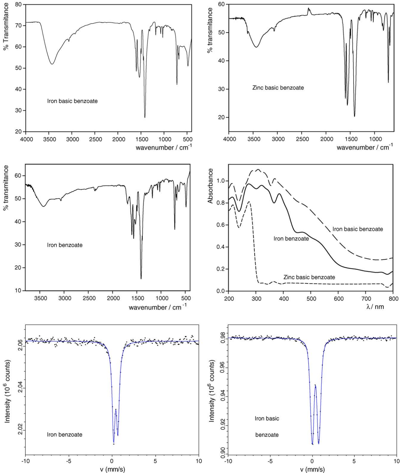
Fig. 6. UV-vis diffuse reflectance, FTIR and Mössbauer spectra of zinc basic benzoate and iron benzoates.
