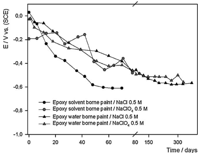
Fig. 10. Corrosion potential of coated steel in 0.5 M NaClO 4 and 3% NaCl.
