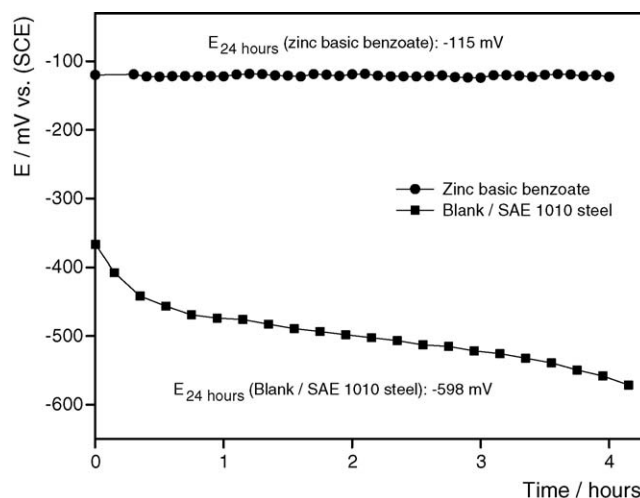
Fig. 3. Corrosion potential of SAE 1010 steel in zinc basic benzoate in 0.5 M \text{NaClO}_4 suspensions.
