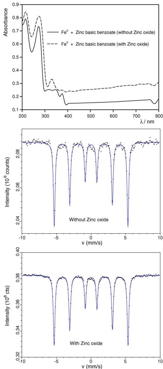
Fig. 7. UV–vis diffuse reflectance, FTIR and Mössbauer spectra of the iron/zinc basic benzoate mix.
