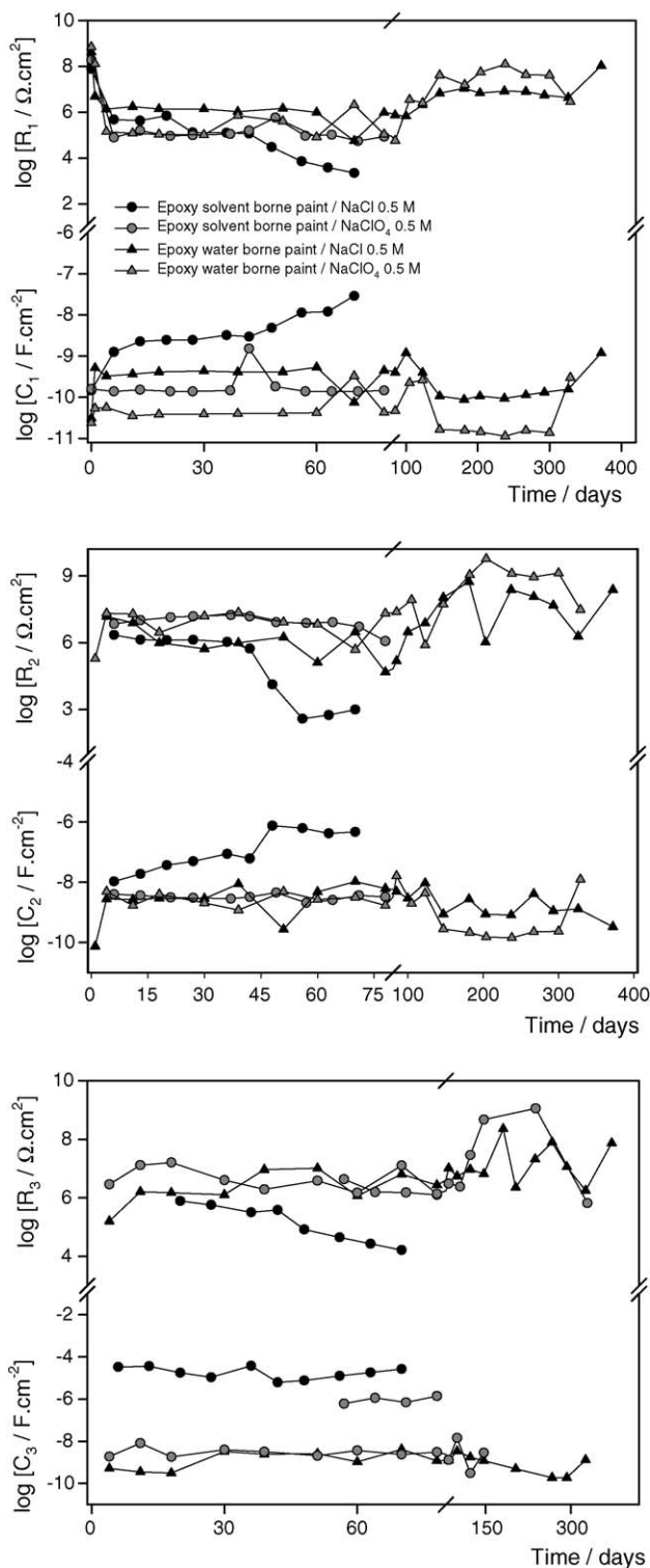
Fig. 11. Fitting parameters, R_i and C_i , for the different coatings, as a function of the immersion time in 0.5 M NaClO 4 and 3% NaCl.
