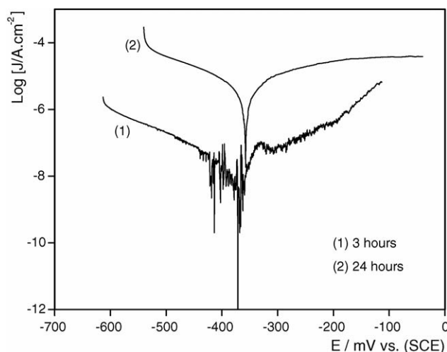
Fig. 4. Tafel plots of the SAE 1010 steel electrode in zinc basic benzoate suspensions in 0.5 M \text{NaClO}_4 , at different exposure times.
