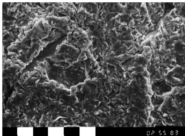
Fig. 5. SEM micrograph of the steel surface after being in contact 24 h with zinc basic benzoate suspension in 0.025 M \text{NaClO}_4 (magnification 1000 \times ).
