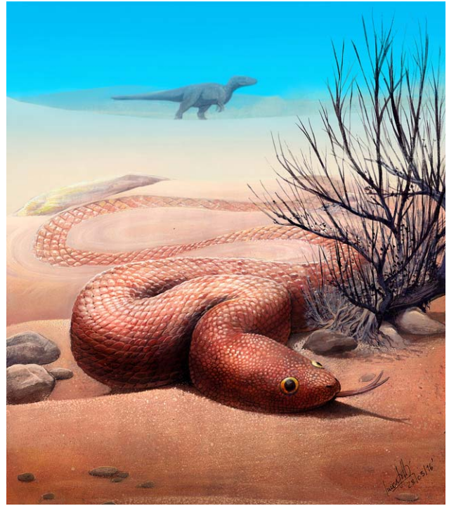
Fig. 12. Reconstruction of Dinilyisia patagonica .
