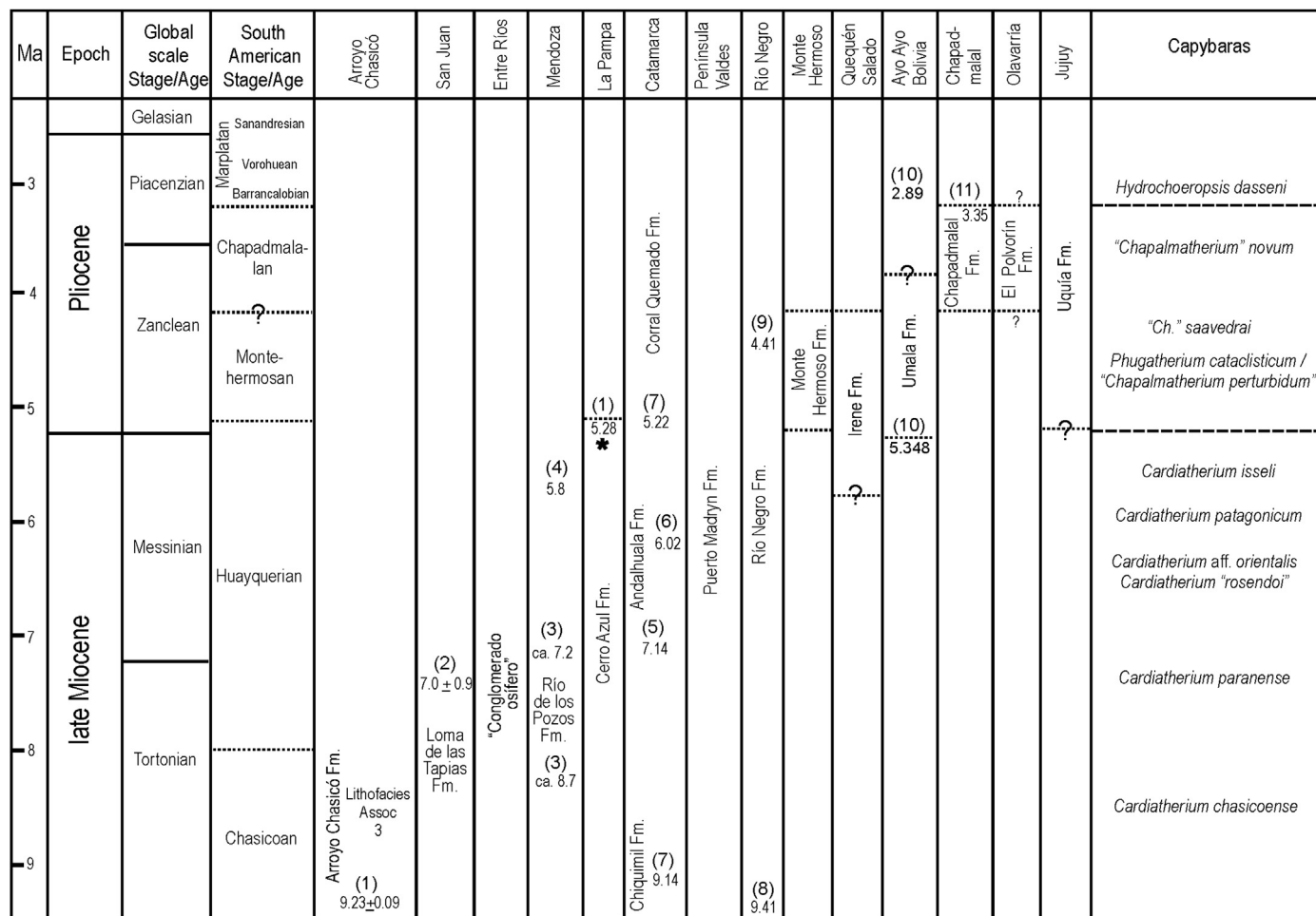
Fig. 5. Stratigraphic chart with correlation of units bearing capybaras with Global and South American stages/ages. (1) Schultz et al., 2006; Zárate et al., 2007; (2) Bercowsky et al., 1986; Serafini et al., 1985; (3) Irigoyen et al., 2002; (4) Marshall et al., 1986; (5) Latorre et al., 1997; (6) Marshall and Patterson, 1981; (7) Bossi and Muruaga, 2009; (8) Zinsmeister et al., 1981; (9) Alberdi et al., 1997; (10) Marshall et al., 1992; (11) Schultz et al., 1998. * This formation sensu Folguera and Zárate (2009), exposed at Cantera Vialidad, near Bahía Blanca.
