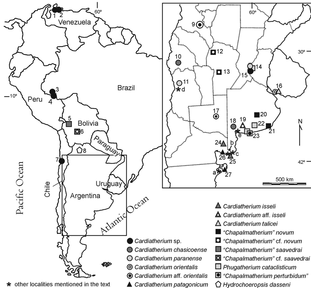
Fig. 1. Location map showing localities bearing Mio-Pliocene capybaras, and the recorded taxa. 1, Urumaco River; Venezuela; 2, San Gregorio, Venezuela; 3, Juruá River, Brazil; 4, Acre River, Perú; 5, Ayo Ayo, Bolivia; 6, Inchasi, Bolivia; 7, Bahía Inglesa, Chile; 8–15, 17–27, Argentina. 8, Uquía, Jujuy; 9, Andalhuala, Catamarca; 10, Albardón, San Juan; 11, Tupungato, Mendoza; 12, Cantera Tuclame (La Playa), Córdoba; 13, Cantera Maero (Las Caleras), Córdoba; 14, Paraná River cliffs, Paraná City, Entre Ríos; 15, La Juanita, Entre Ríos; 16, Barrancas de San Gregorio, Uruguay; 17, Laguna Chillhué and Laguna Guatraché, La Pampa; 18–22, Buenos Aires Province. 18, Arroyo Chasicó, 19, Sauce Grande River; 20, Calera Avellaneda; 21, Chapadmalal; 22, Quequén Salado River; 23, Farola Monte Hermoso; 24–26, Río Negro Province. 24, General Conesa; 25, Bahía Creek; 26, Balneario La Lobería; 27, Rincón Chico – La Pastosa (Chubut). a–e, other localities mentioned in the text. a, Punta Cracker; b, Balneario El Cóndor – Bahía Rosas; c, mouth of the Río Negro River; d, Huayquerías de San Carlos; e, Cantera Vialidad.
