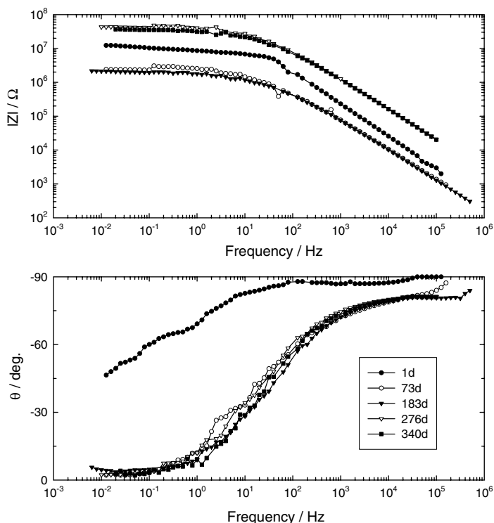
Fig. 14. Bode plots, at different exposure times, for paint 3 in 0.5 M NaClO 4 .
