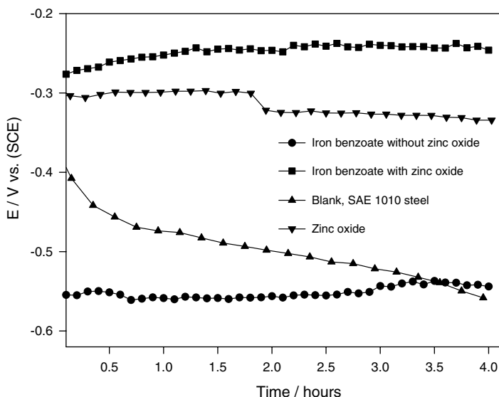
Fig. 2. Corrosion potential of SAE 1010 steel in ferric benzoate suspensions in 0.5 M \text{NaClO}_4 .
