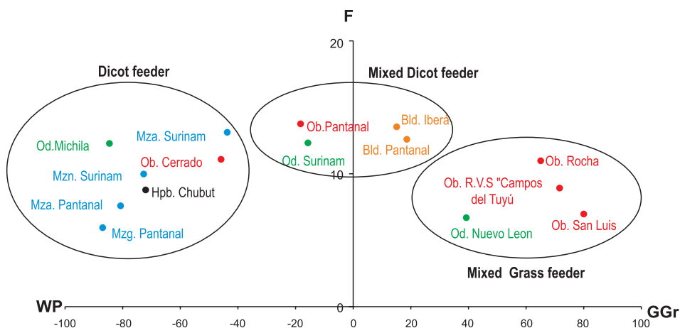
Figure 3 - Annual diet of different population of six species of Neotropical deer represented within a triangle. The composition of annual diet in terms of percentage of Woody Plants (WP), Forbs (F) and Grasses and Graminiforms (GGr). In a circle different plant food preference followed Spencer (1995). Ob.: Ozotoceros bezoarticus , Bld.: Blastocerus dichotomus , Mza.: Mazama americana , Mzg.: Mazama gouazoubira , Mzn.: Mazama nemorivaga and Od.: Odocoileus virginianus .
