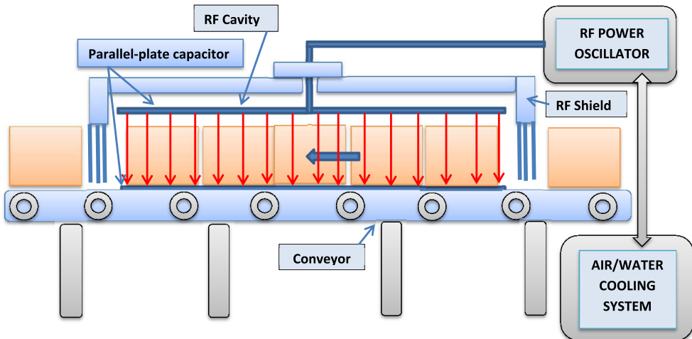
Fig. 3. Schematics of a conveyORIZED RF processing system.
