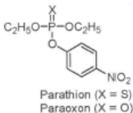
Fig. 6. Chemical structure of parathion and paraoxon.
